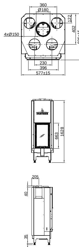
Linear Front 39x66 (P. 48) Arte 1Vh-66-4S
