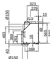
Swing Insert 81x54 (P. 66) Linear XL
