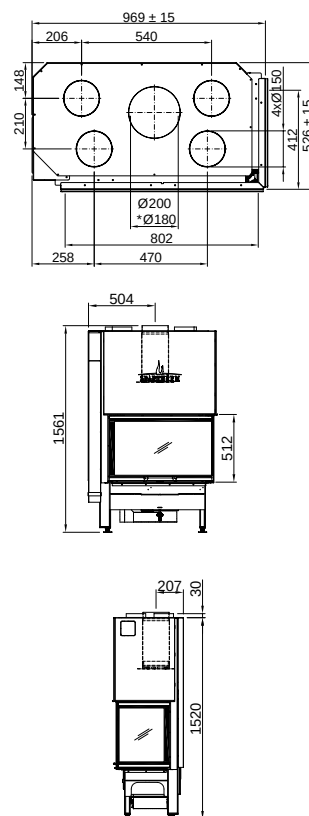
Linear Corner 80x40x50 (P. 44) Varia 2L/2R-80h-4S
