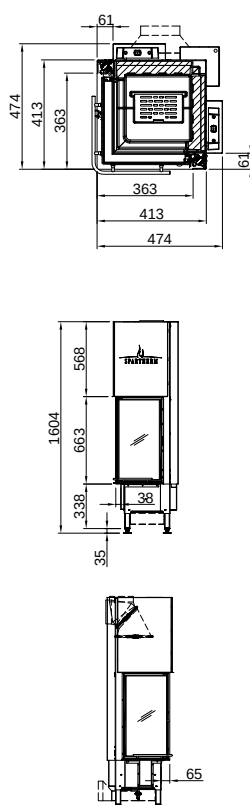
Linear Corner 36x36x66 (P. 38) Arte 2LRh-66-4S
