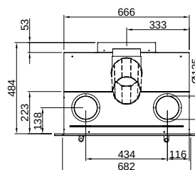
Swing Insert 61x50 (P. 66) Linear M
