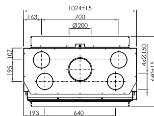
Premium Tunnel 87x50 (P. 60) Premium V-FD-87h
