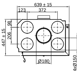
Swing Corner 58x39x51 (P. 40) Varia 2L/2R-55-4S
