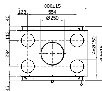
Swing Tunnel 67x51 (P. 62) Varia FD-4S
