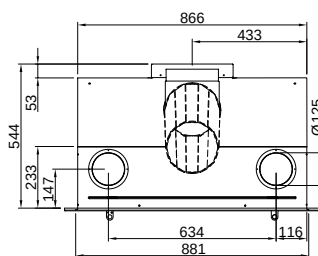
Swing Insert 81x54 (P. 66) Linear XL
