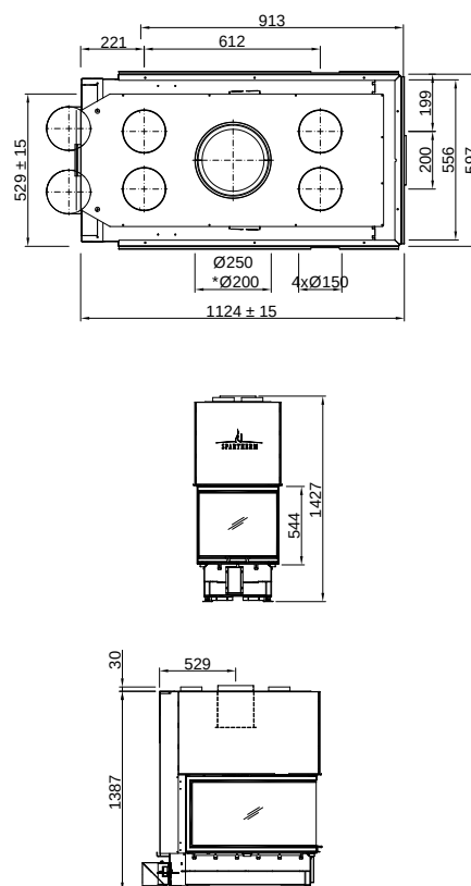
Linear Triple 55x91x54 (P. 34) Arte U-90h-4S
