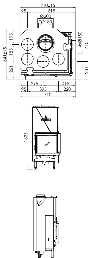
Linear Corner 36x36x66 (P. 38) Arte 2LRh-66-4S
