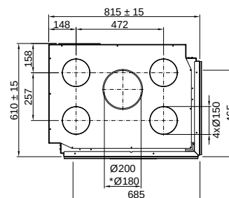
Linear Corner 68x46x51 (P. 42) Varia 2Lh/2Rh-51-4S
