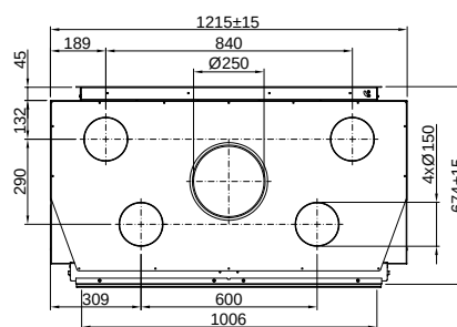
Linear Tunnel 100x52 (P. 64) Varia B-FDh-4S
