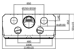
Linear Front 100x70 (P. 58) Varia 1V-100h-4S
