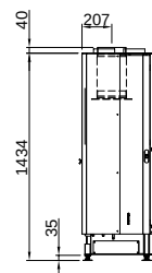
Linear Front 88x44 (P. 56) Varia Ah-4S
