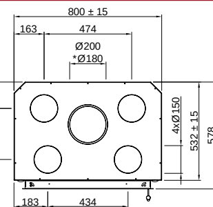
Swing Front 67x57 (P. 52) Varia 1V-57-4S
