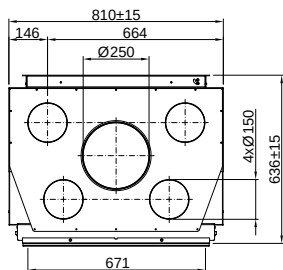
Linear Tunnel 67x57 (P. 62) Varia FDh-57-4S
