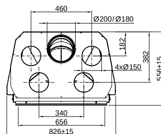
Linear Front 65x80 (P. 50) Arte Bh-4S
