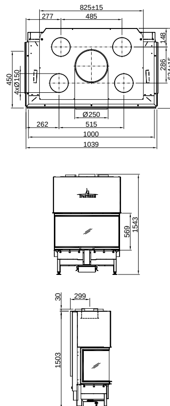
Linear Triple 100x45x56 (P. 32) Arte 3RL-100h-4S
