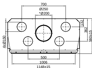
Linear Front 100x51 (P. 58) Varia Bh-4S
