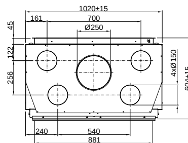
Linear Tunnel 88x44 (P. 64) Varia A-FDh-4S
