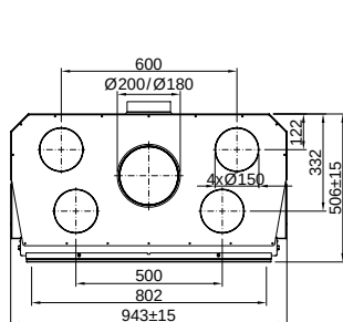
Linear Front 80x52 (P. 56) Varia M-80h-4S
